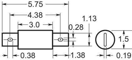
110 to 200 A
